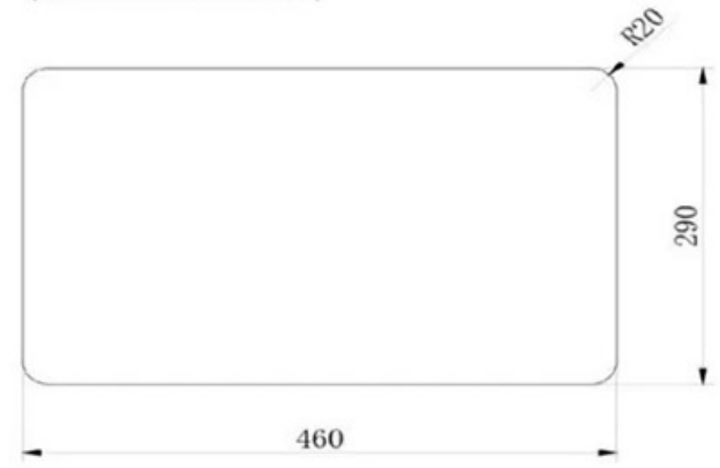
Cutting Size (Undermounted Installation)
