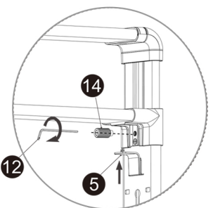
2.4. Fasten the screws and screw cap to the frame
