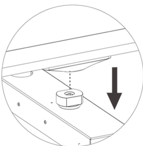
2.1. Attach the frame to the revolving base
