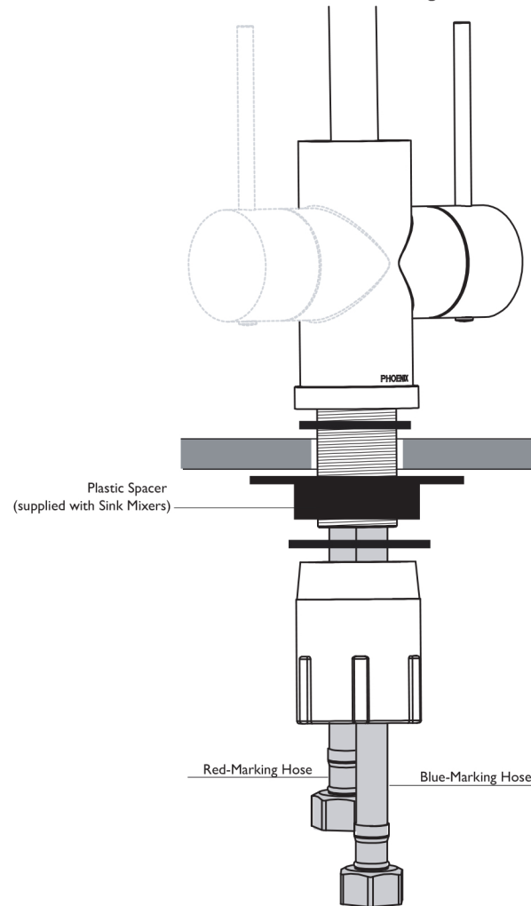
SIDE LEVER MIXER - Single/Twin Handle
