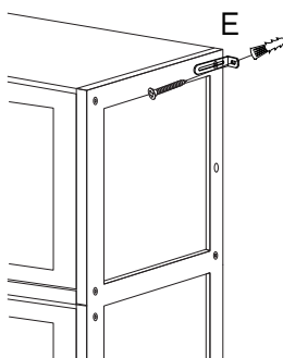
Wall-locked installation
