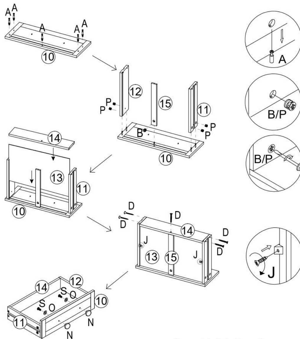
Assemble 3 bottom drawers
