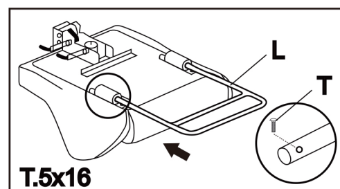
6. Insert footrest chassis to holder
