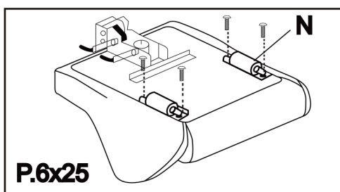
5. Install footrest plate holder
