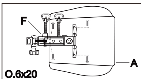
4. Install seat plate to under cushion
