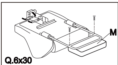
7. Install footrest cushion to chassis
