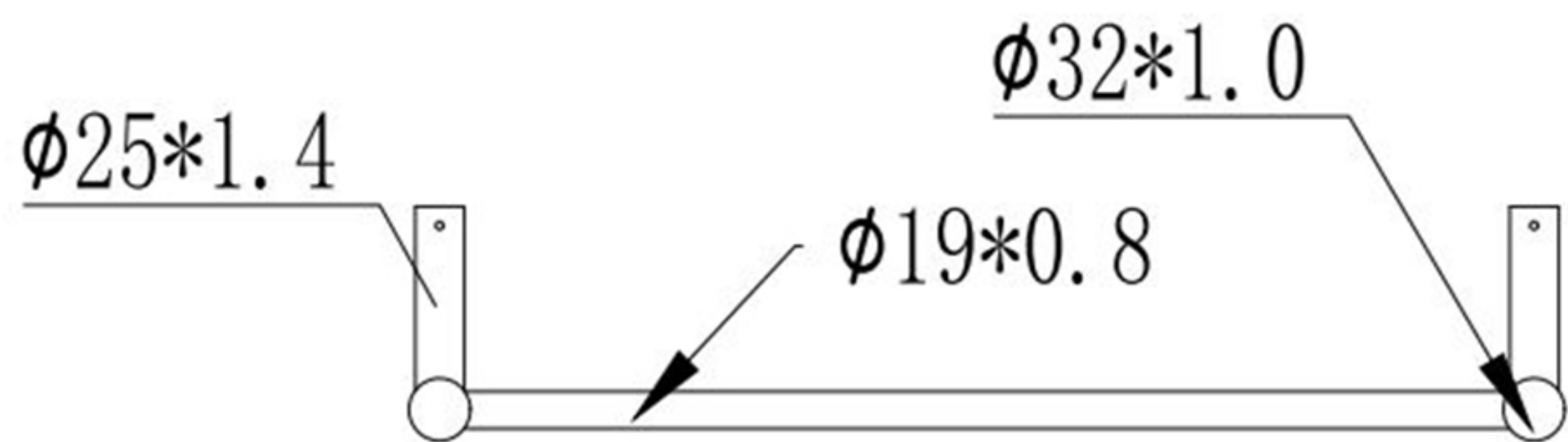
Top View
