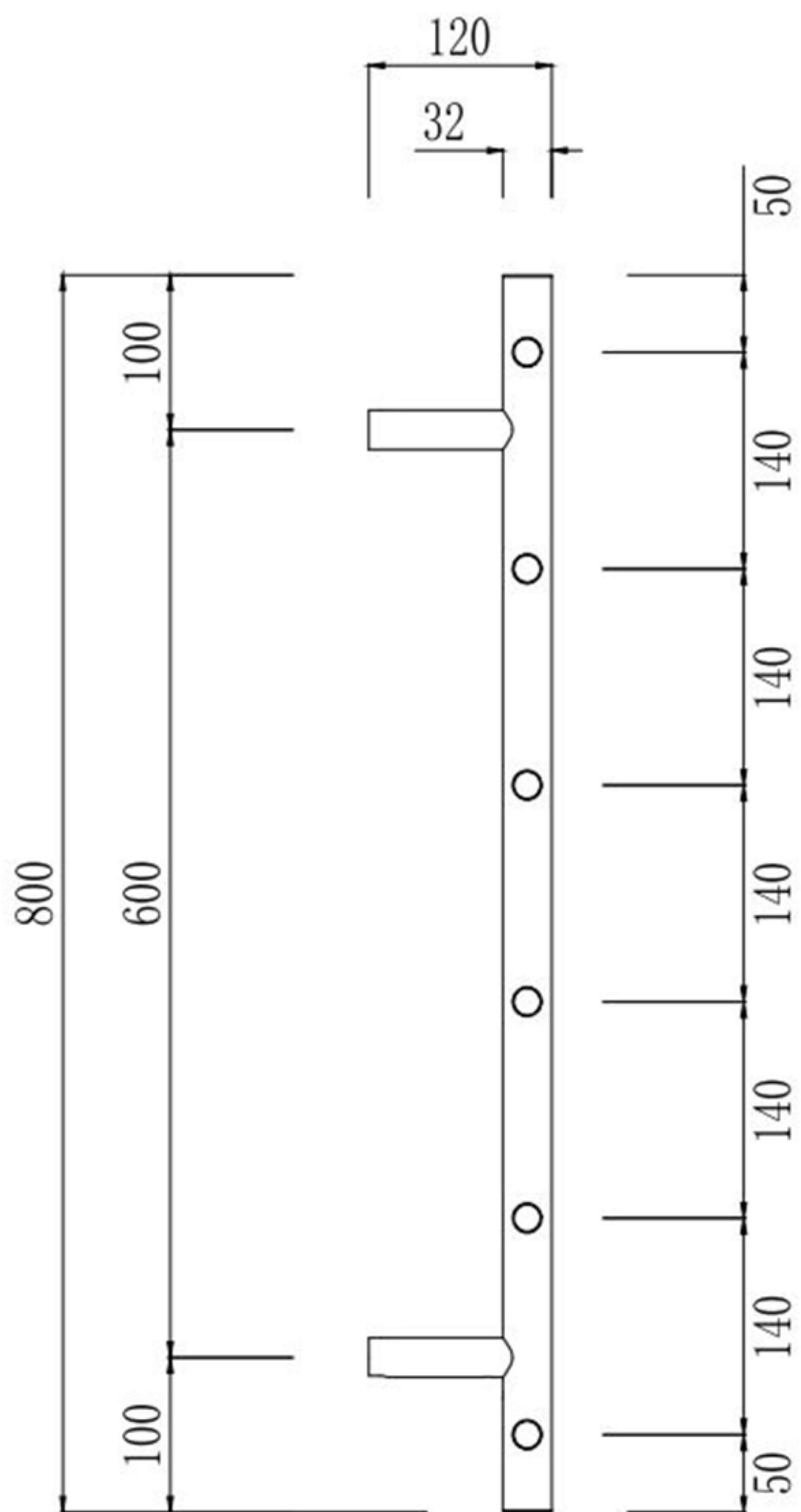
Side View
