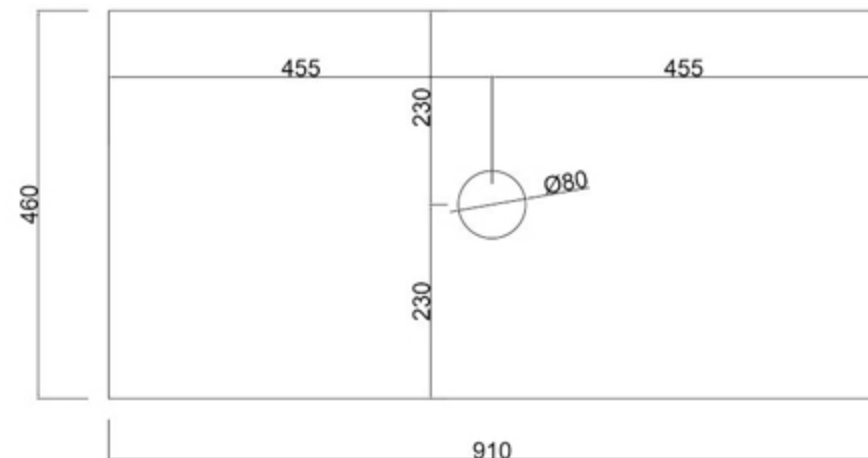
TOP VIEW W/ QUARTZ
