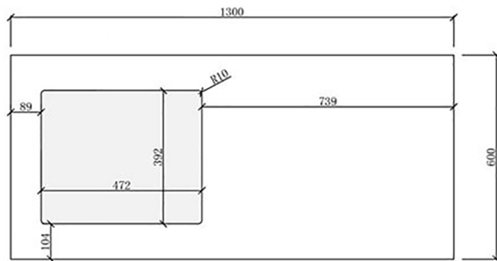
Top View
