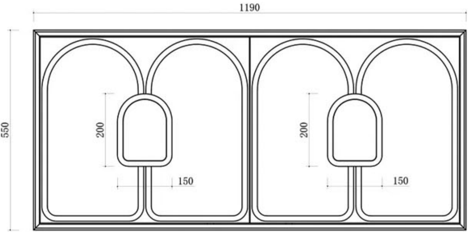
Front View
