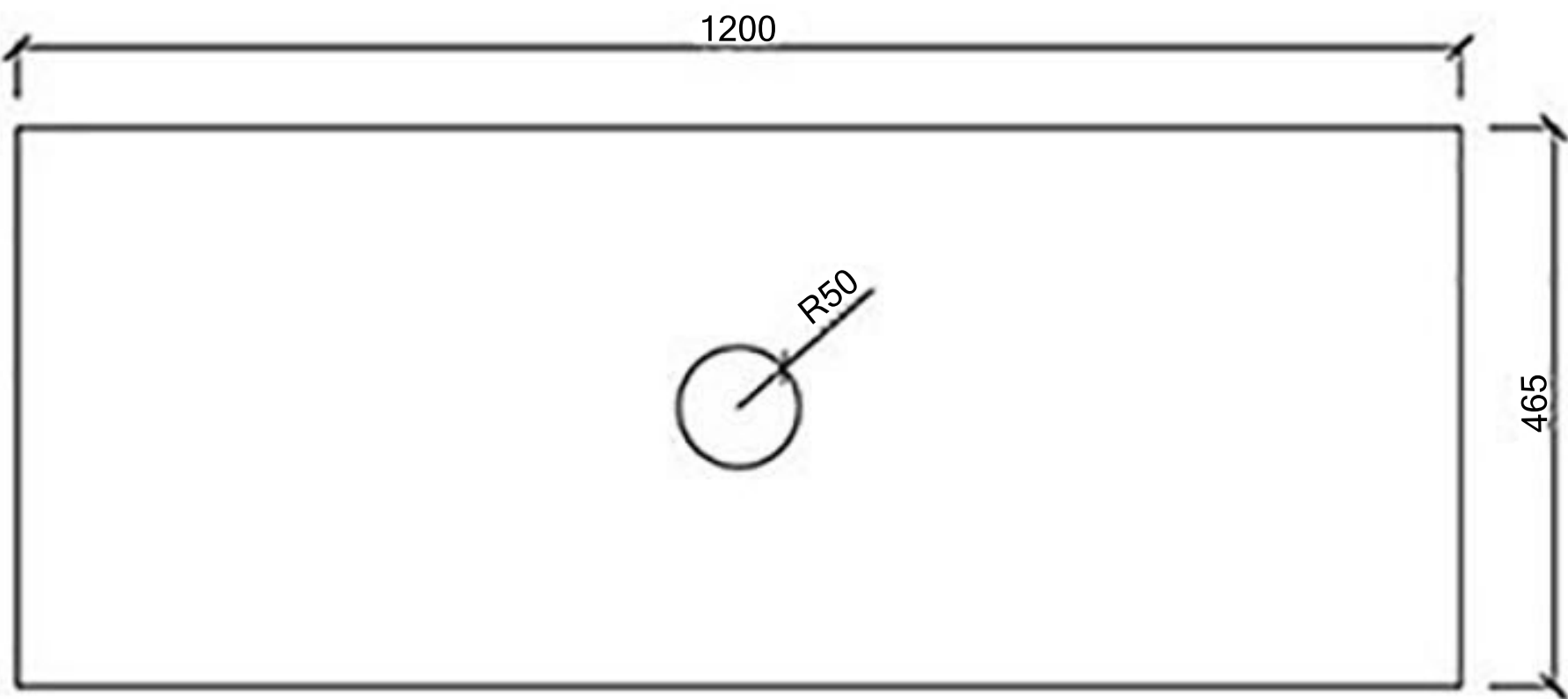
Front View
