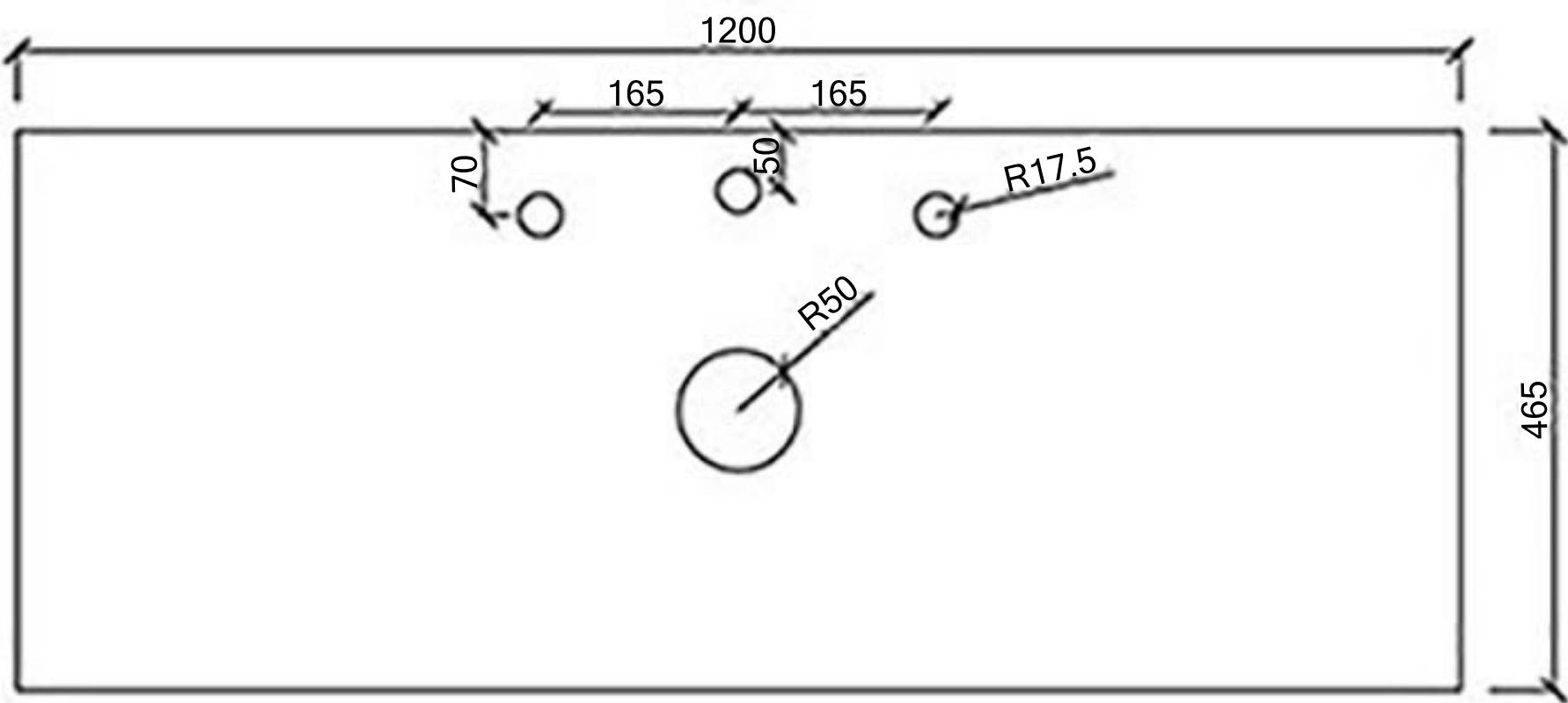
Back View Pre Semi-Drilling Tophole
