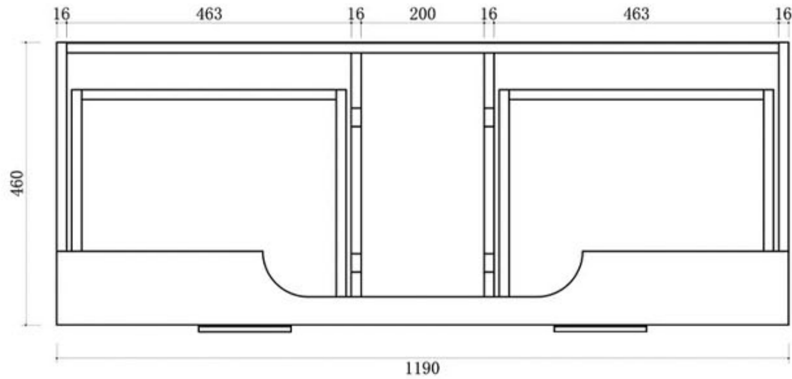
Top View
