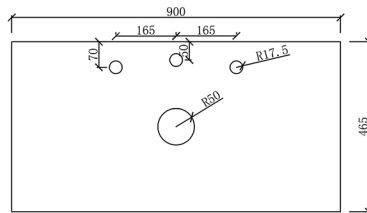
Back View Pre Semi-Drilling Taphole
