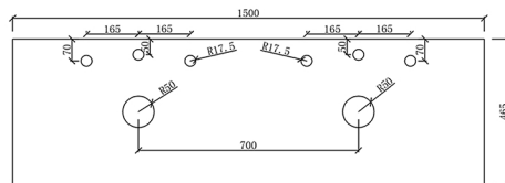
Back View Pre Semi-Drilling Taphole
