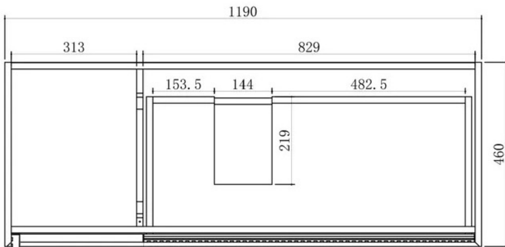
Top View
