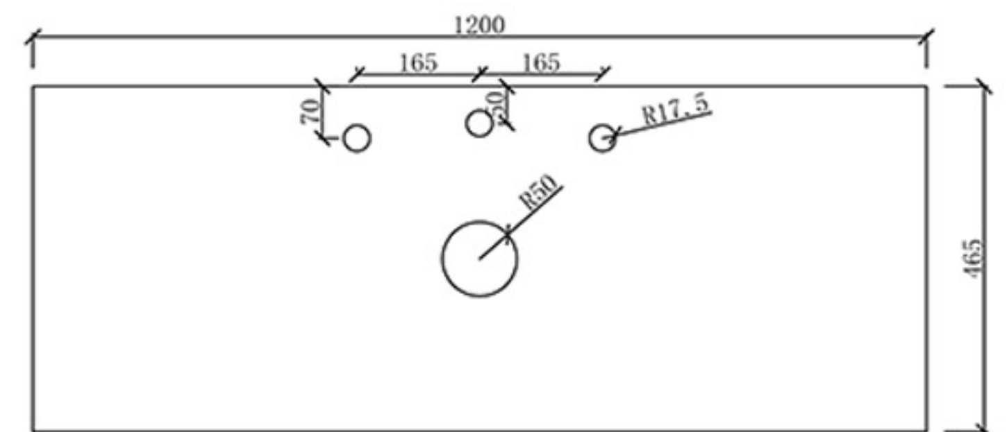
Back View Pre Semi-Drilling Taphole
