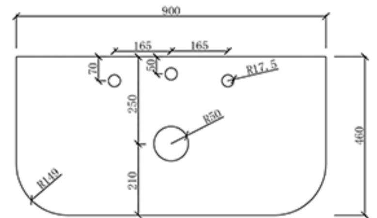
Back View Pre Semi-Drilling Tophole
