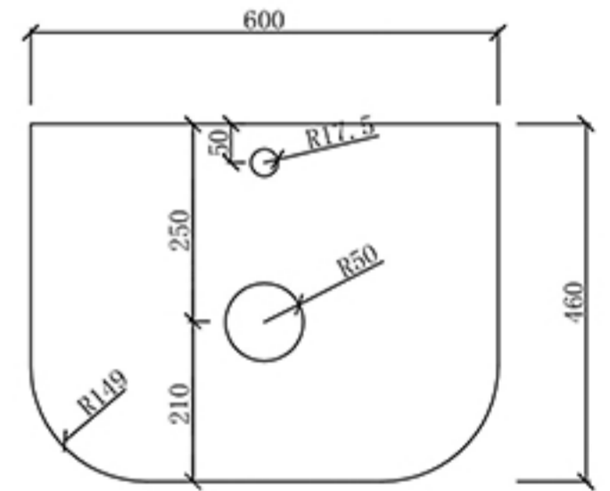
Back View Pre Semi-Drilling Taphole
