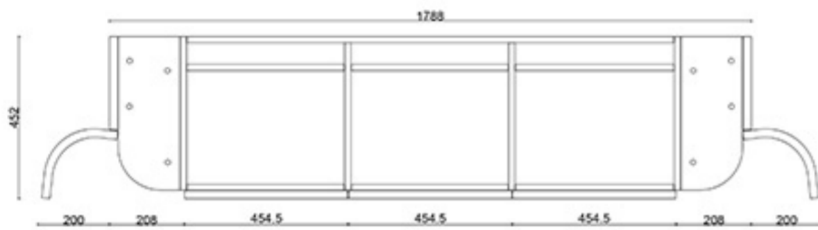
TOP VIEW
