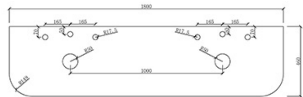
Back View Pre Semi-Drilling Tophole
