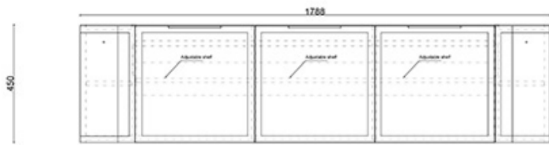
FRONT VIEW
