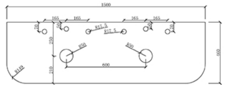
Back View Pre Semi-Drilling Tophole
