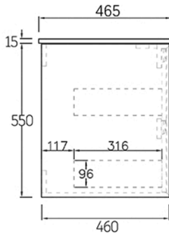
Side View
