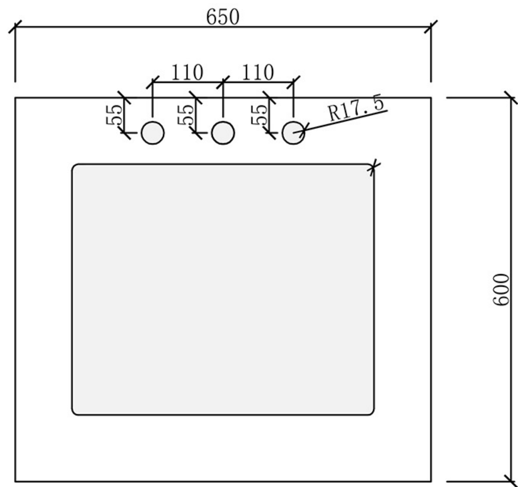
Back View Pre Semi-Drilling Tapholes
