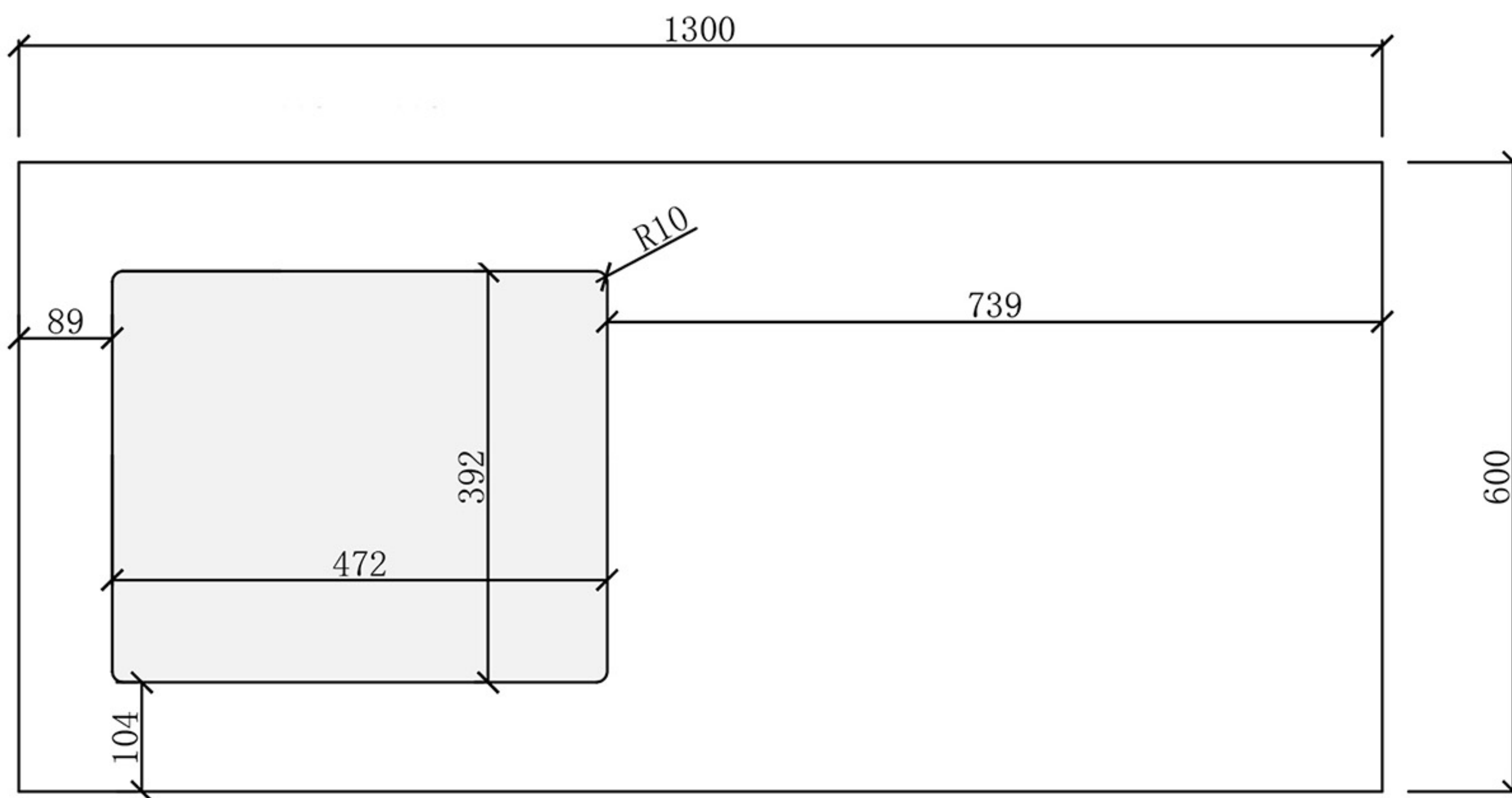
Top View
