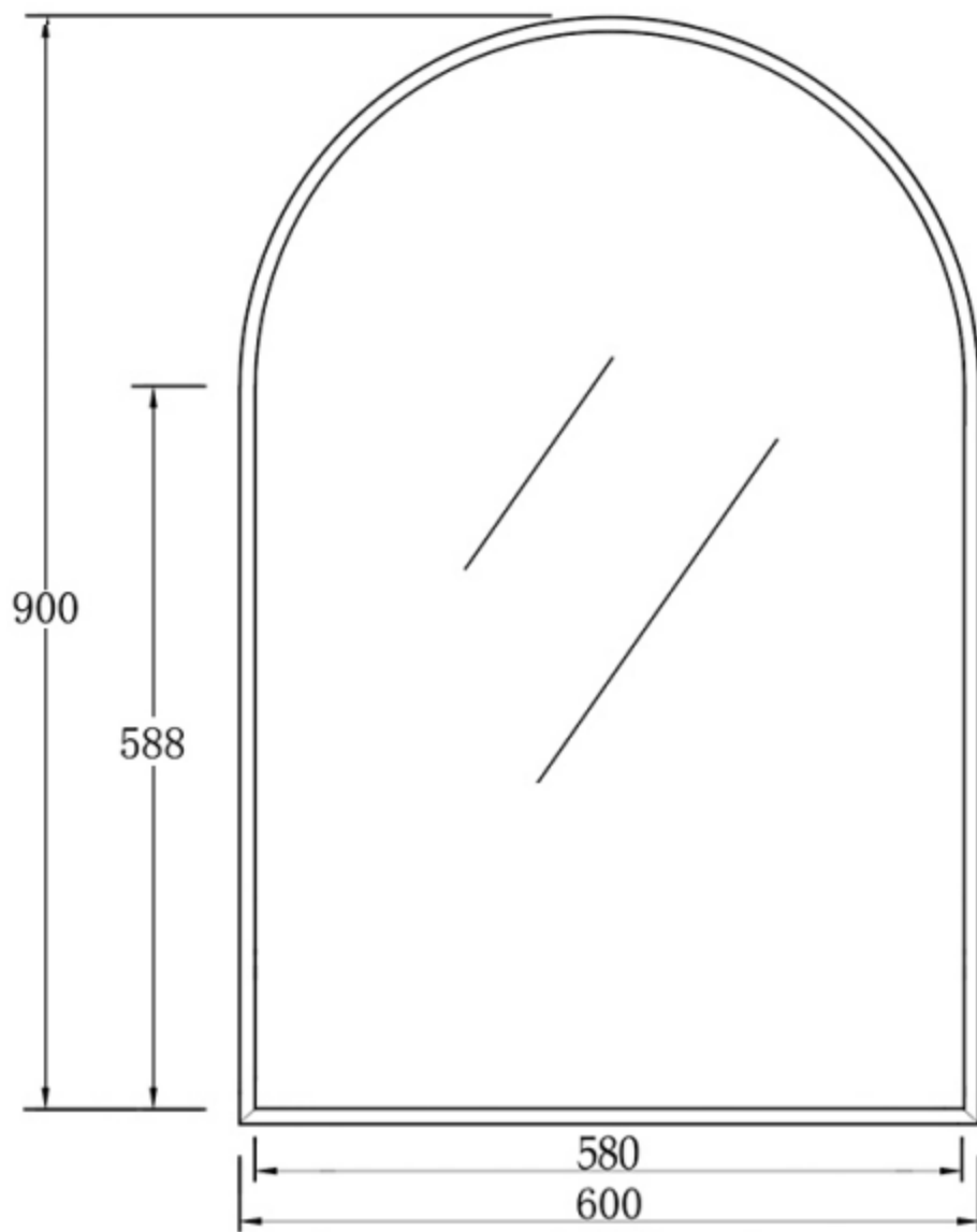
FRONT VIEW
