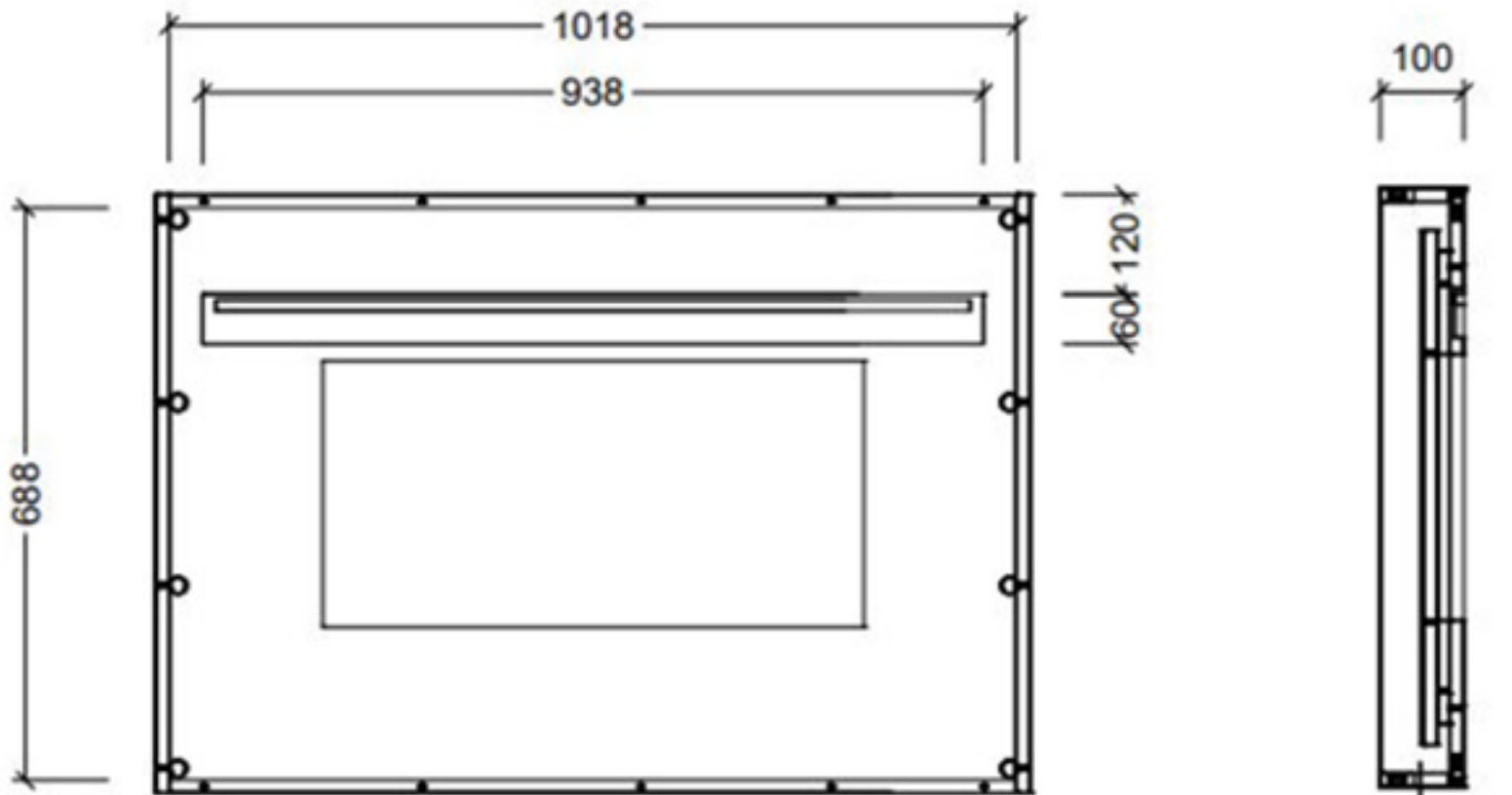
BACKING BOARD
