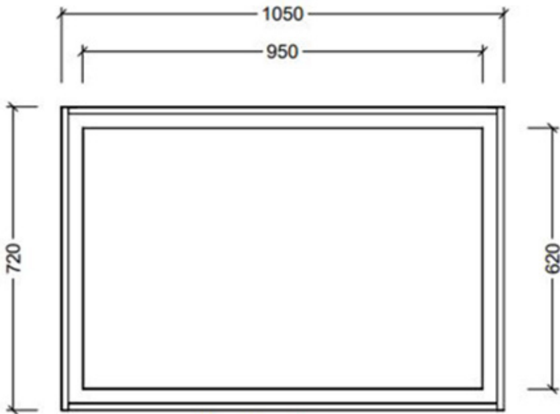
MIRROR / FRAME
