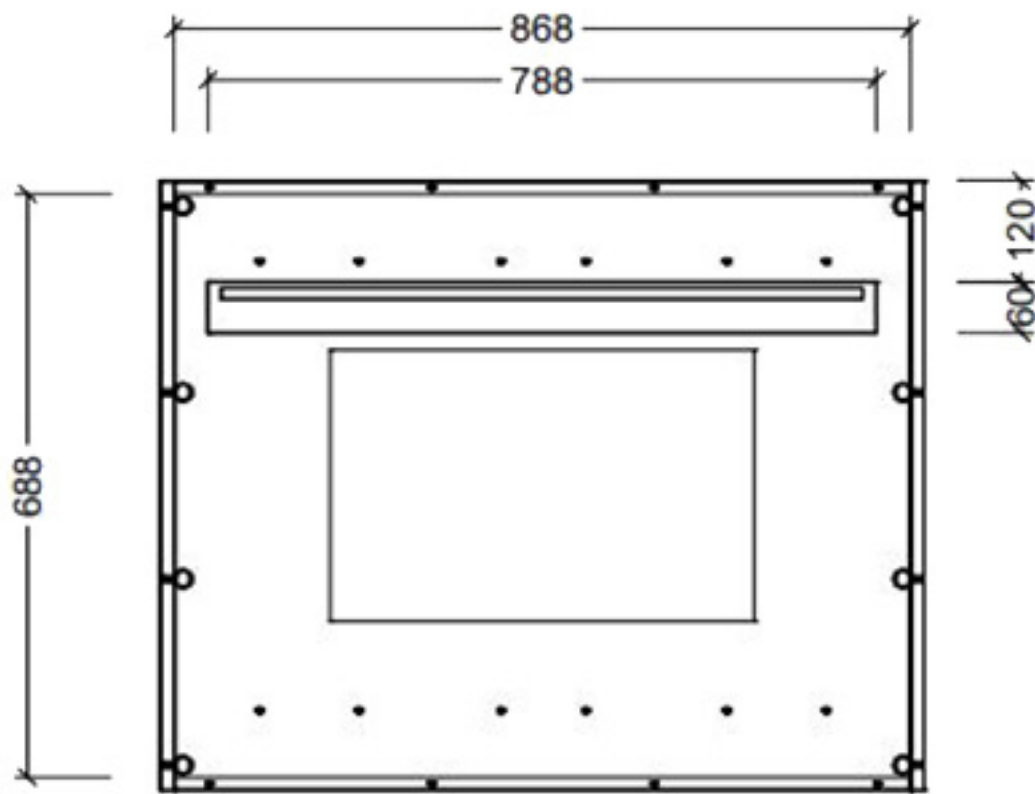
BACKING BOARD
