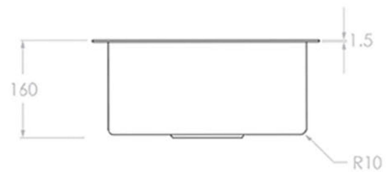
INNER SINK
