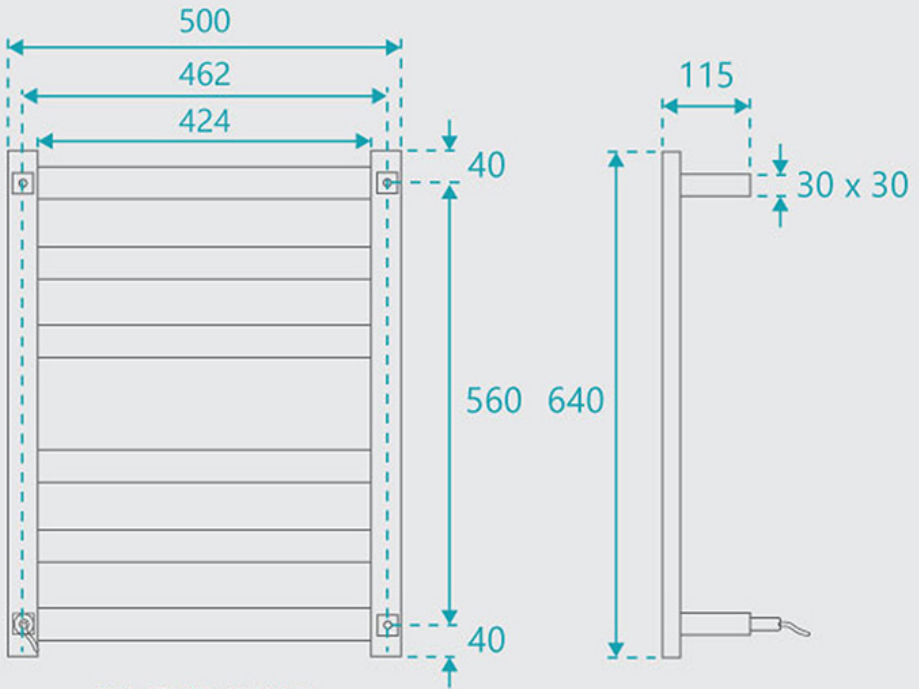
BACK VIEW
