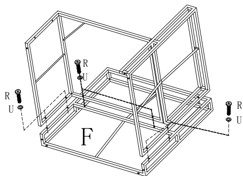
Step 2 Corner sofa 2pcs
