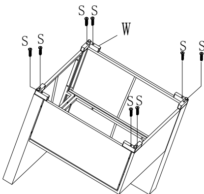
Step 4 Corner sofa 2pcs
