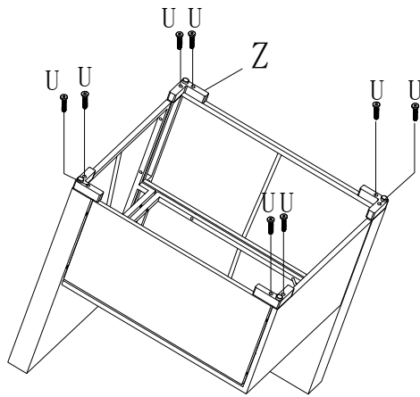
Step 4 Corner sofa 1pc
