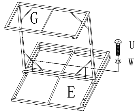
Step 1 Corner sofa 1pc
