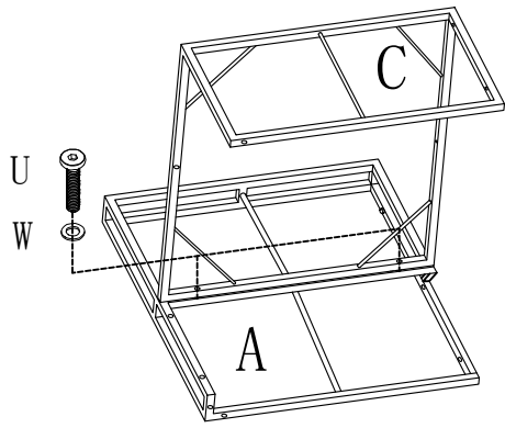
Step 3 Corner sofa 1pc
