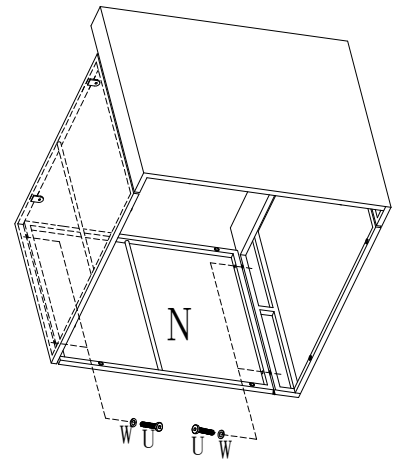
Step 5 Sofa 1pc
