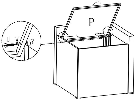
Step 6 Sofa 1pc
