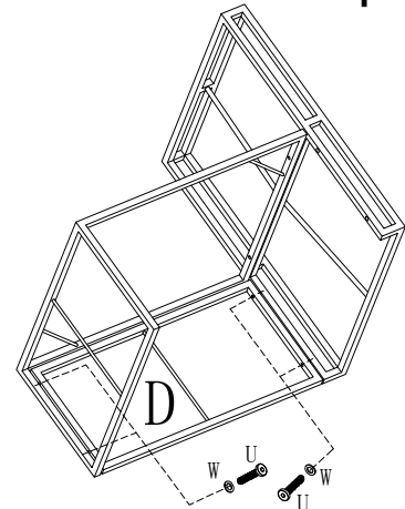
Step 2 Armless sofa 4pcs
