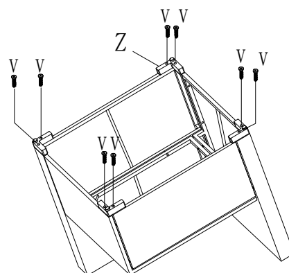
Step 4 Corner sofa 1pc
