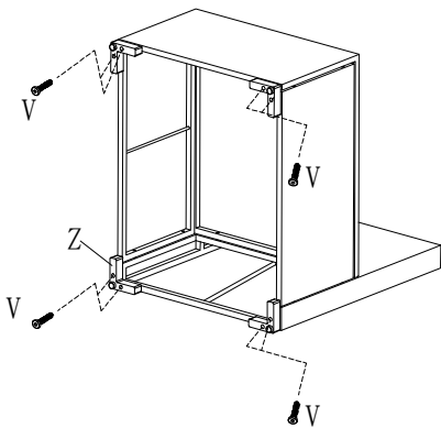
Step 4 Armless sofa 4pcs
