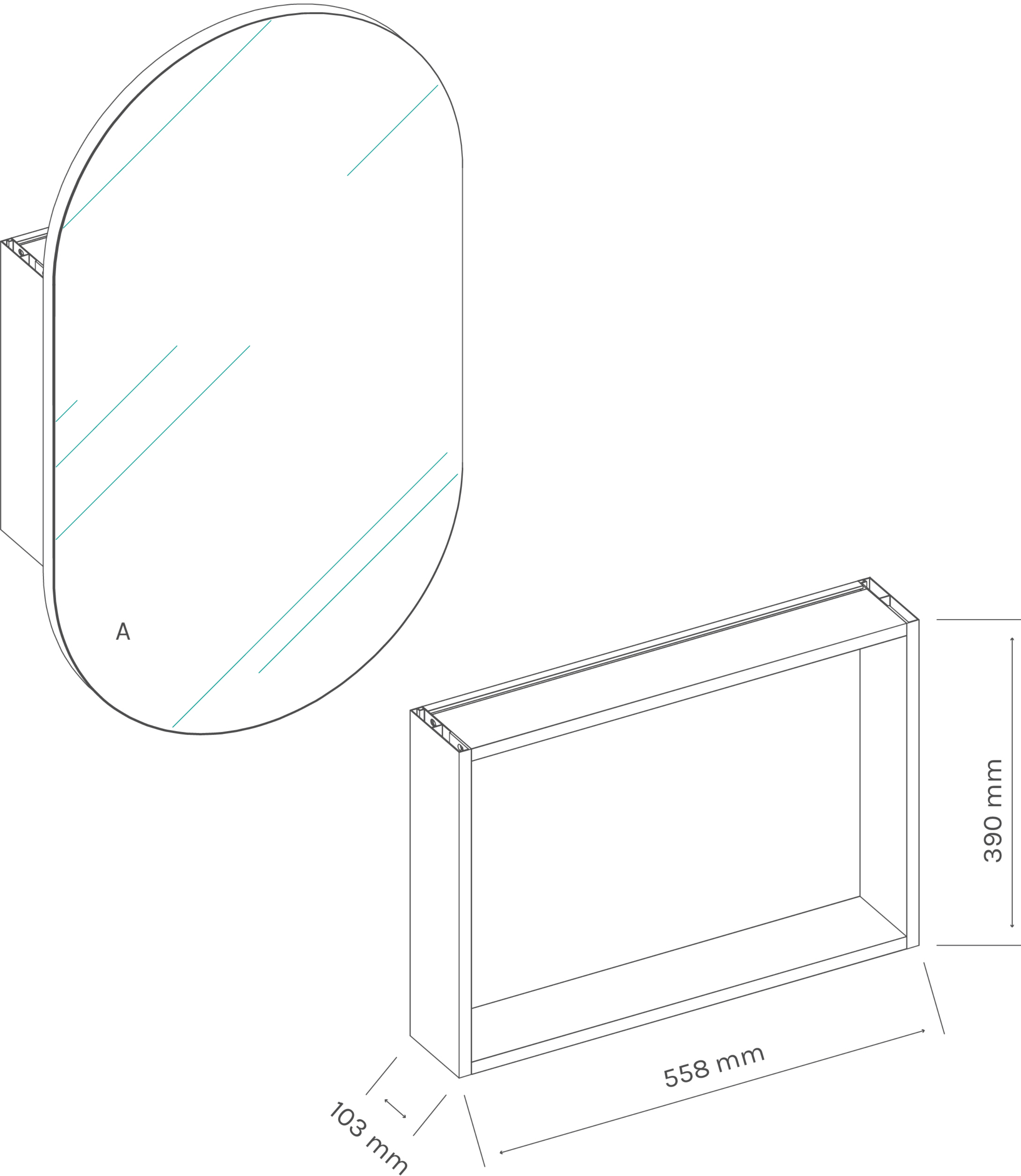
Model FMCP-960X560 (H: 960mm / W: 560mm / 1 Door)
