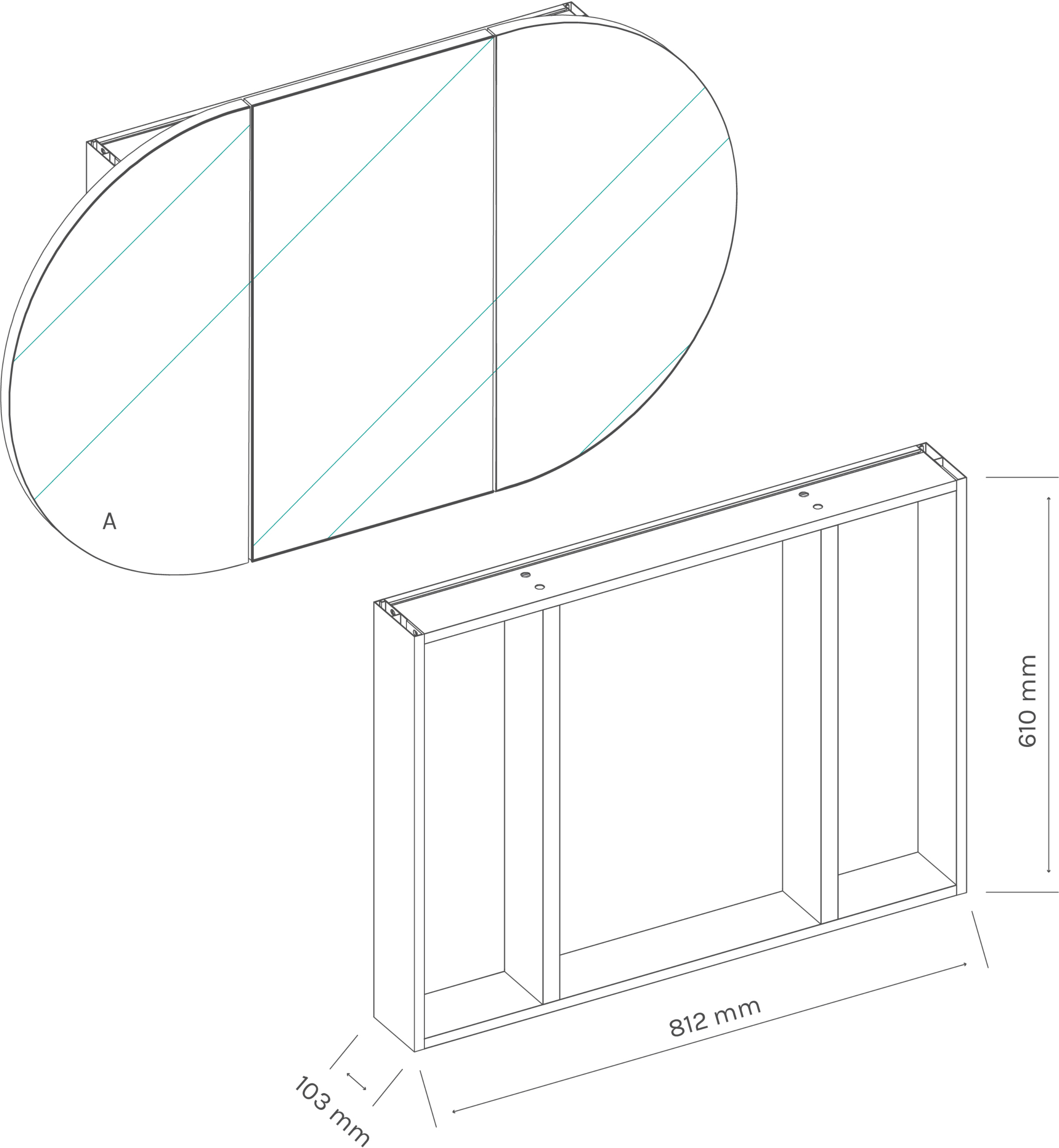
Model FMCP-760X1200 (H: 760mm / W: 1200mm / 3 Doors)
