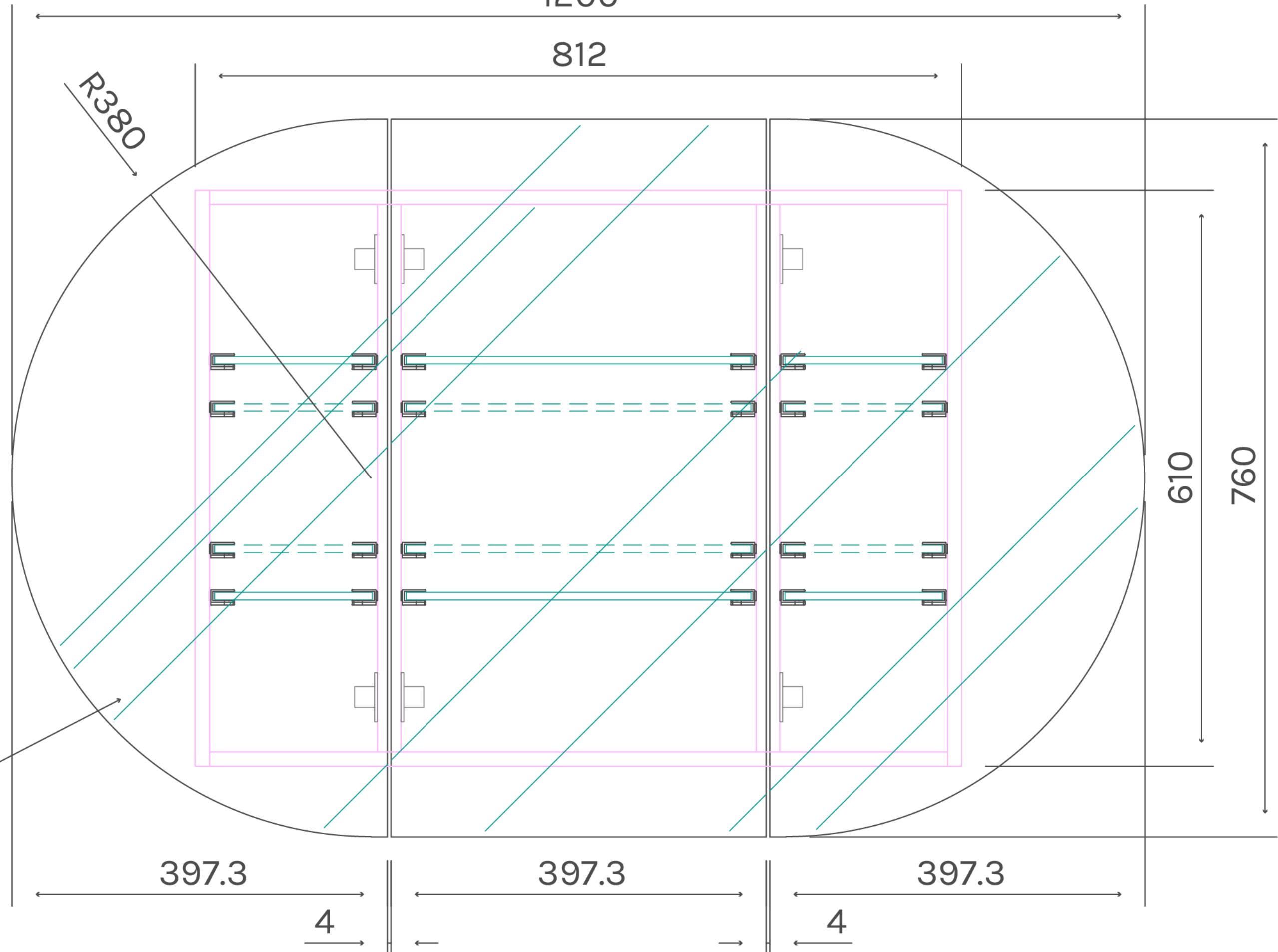
Front view Scale 1:10
