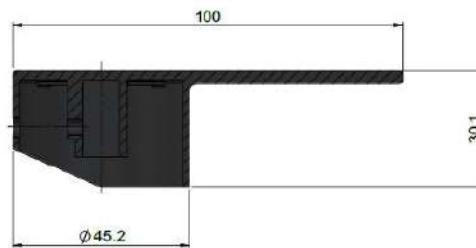
PADDLE HANDLE
