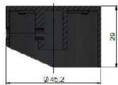
PINLESS HANDLE
