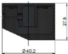
PINLESS HANDLE
