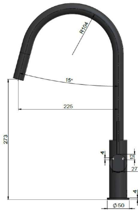
PADDLE HANDLE
