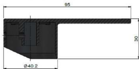
PADDLE HANDLE
