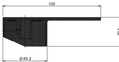
PADDLE HANDLE
