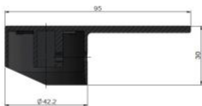
PADDLE HANDLE
