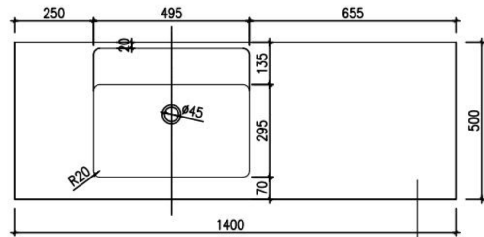
Solid Surface Basin
