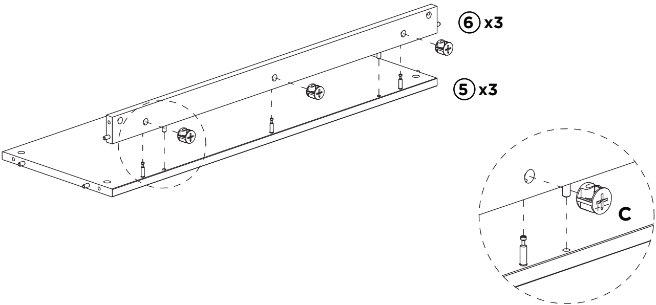
9 Locking Nuts
