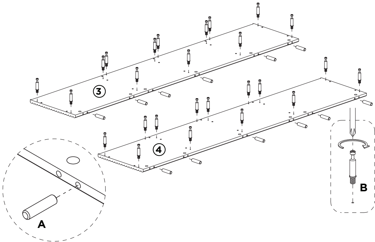
12 Wood Dowels
