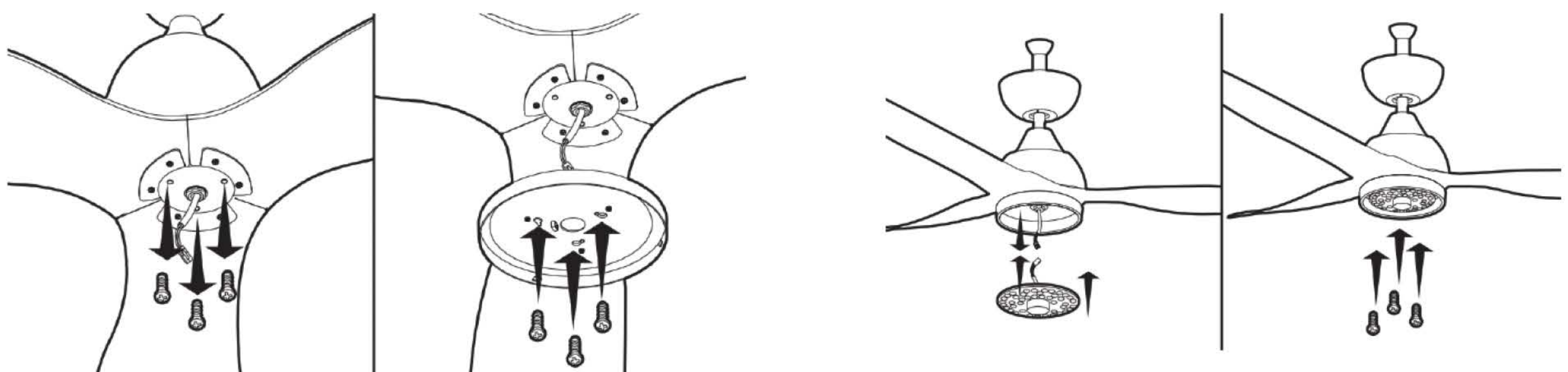
Fg. 7 Fan LED Light Model
