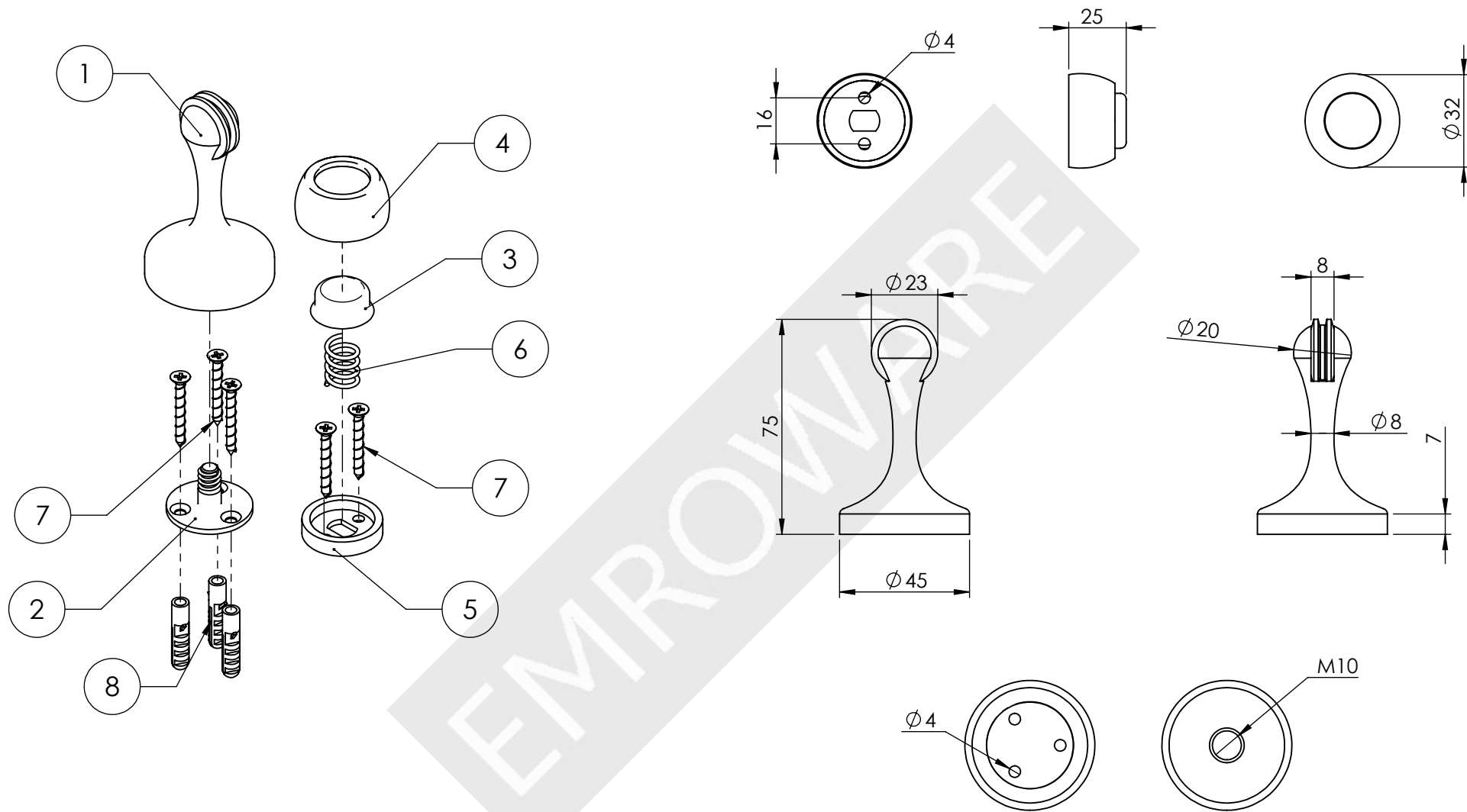
ALTERNATIVE MOUNTING ARRANGEMENTS
