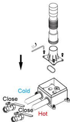
9. Install cleaning parts.
