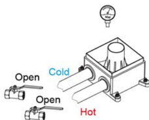
7. Test more than 10 min with 0.8MPA+ water pressure to make sure no leaking.
