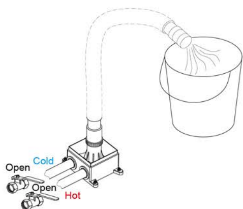
10. Clean the input pipe.
