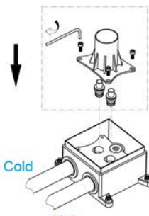
6. Install the sealing part and test the water pressure.
