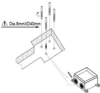
3. Mark the holes and drill dia.8mm holes with D40mm.
