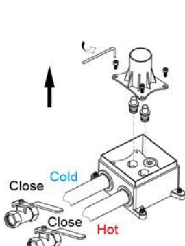
8. Off the water and remove the testing pipe.
