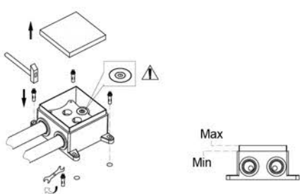
5. Remove the dust cover and adjust it to horizontal and then screw it.
