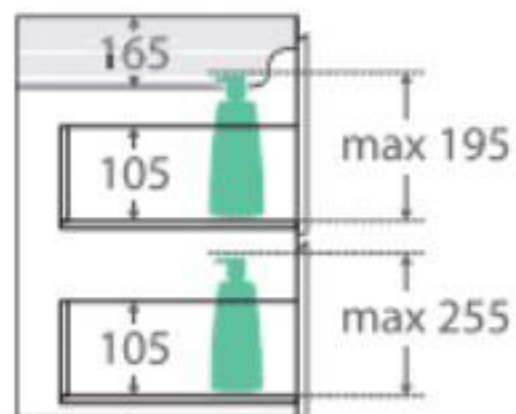
SIDE VIEW: RECESS & DRAWER STORAGE
