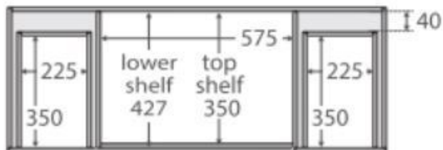
TOP VIEW: SHELF AREA & DRAWER AREA
