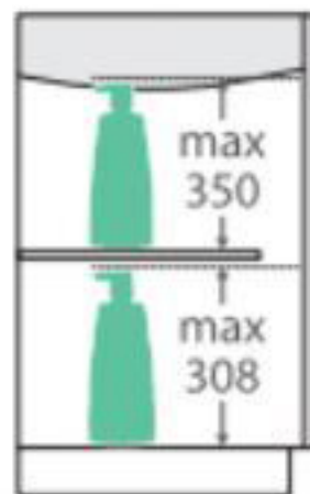
SIDE VIEW: SHELF STORAGE
