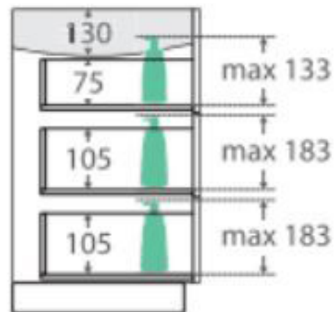
SIDE VIEW: RECESS & DRAWER STORAGE
