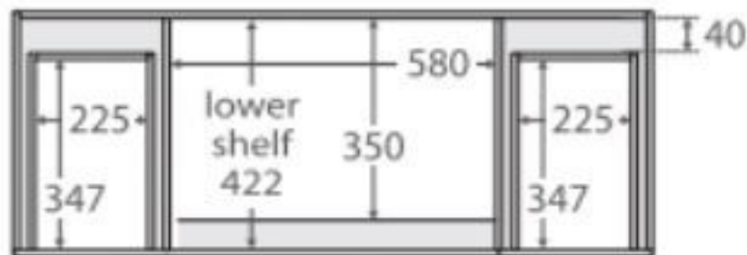
TOP VIEW: SHELF AREA & DRAWER AREA
