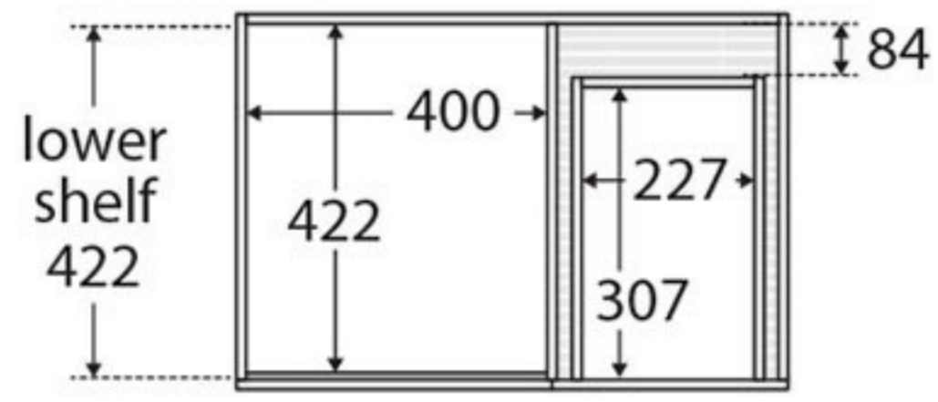
TOP VIEW: SHELF AREA & DRAWER AREA
