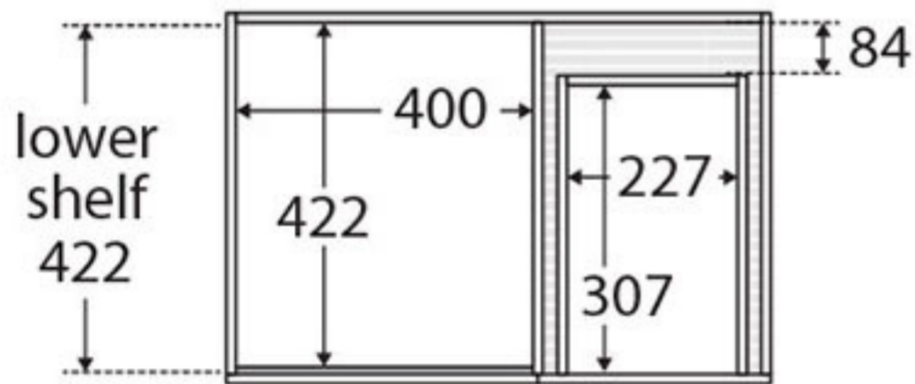
TOP VIEW: SHELF AREA & DRAWER AREA
