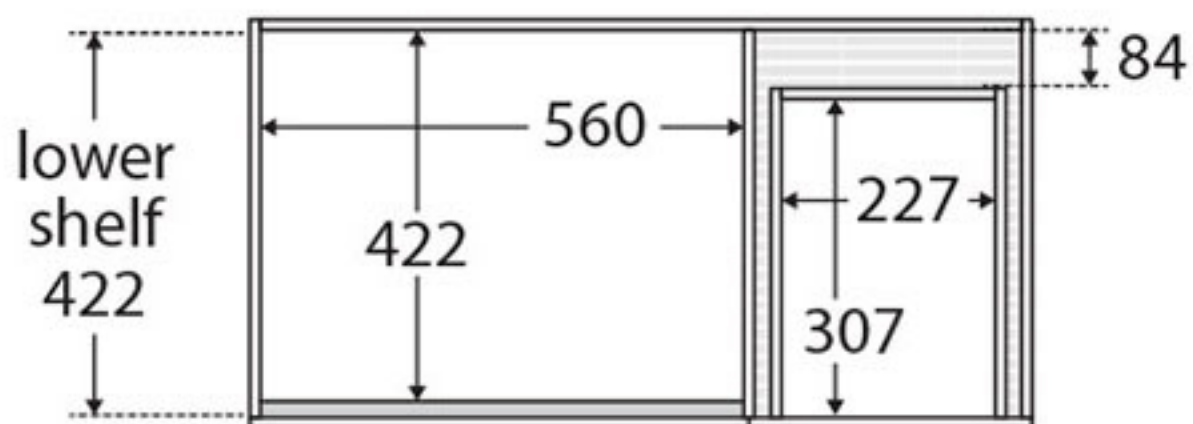
TOP VIEW: SHELF AREA & DRAWER AREA
