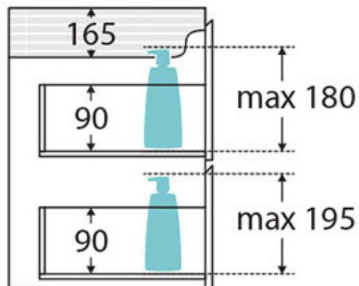
SIDE VIEW: RECESS & DRAWER STORAGE
