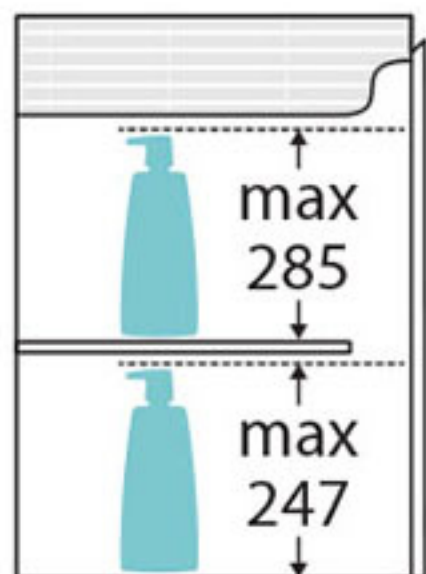
SIDE VIEW: SHELF STORAGE
