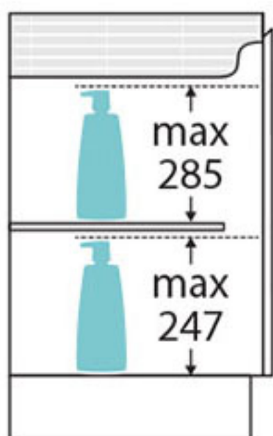
SIDE VIEW: SHELF STORAGE
