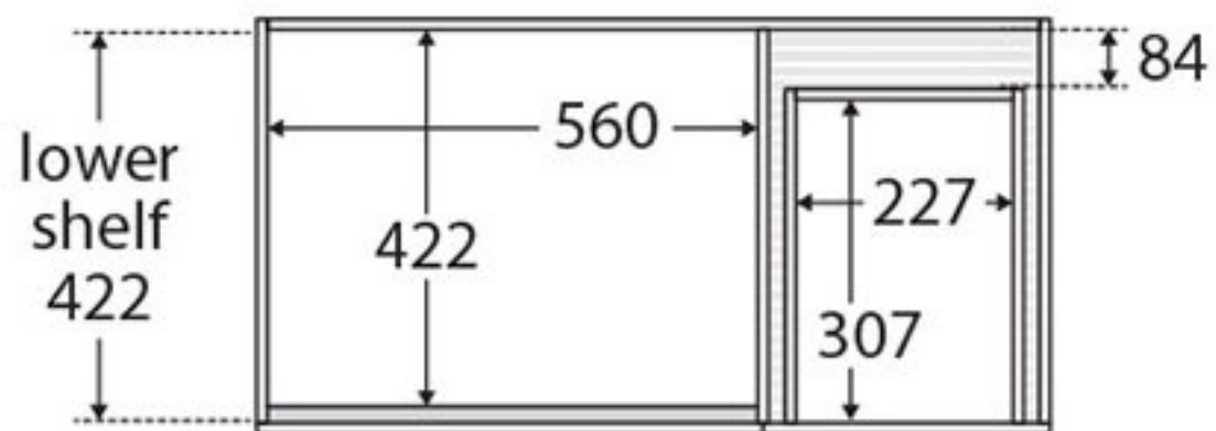
TOP VIEW: SHELF AREA & DRAWER AREA
