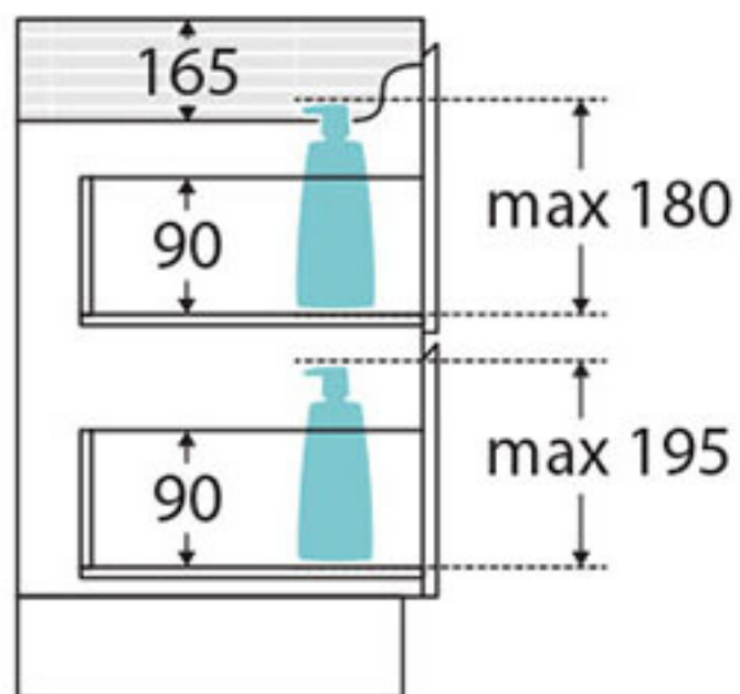
SIDE VIEW: RECESS & DRAWER STORAGE
