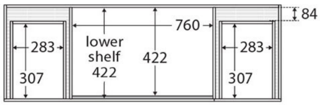
TOP VIEW: SHELF AREA & DRAWER AREA
