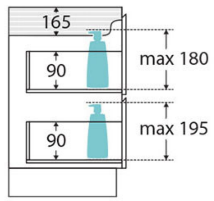
SIDE VIEW: RECESS & DRAWER STORAGE
