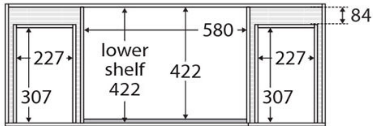
TOP VIEW: SHELF AREA & DRAWER AREA
